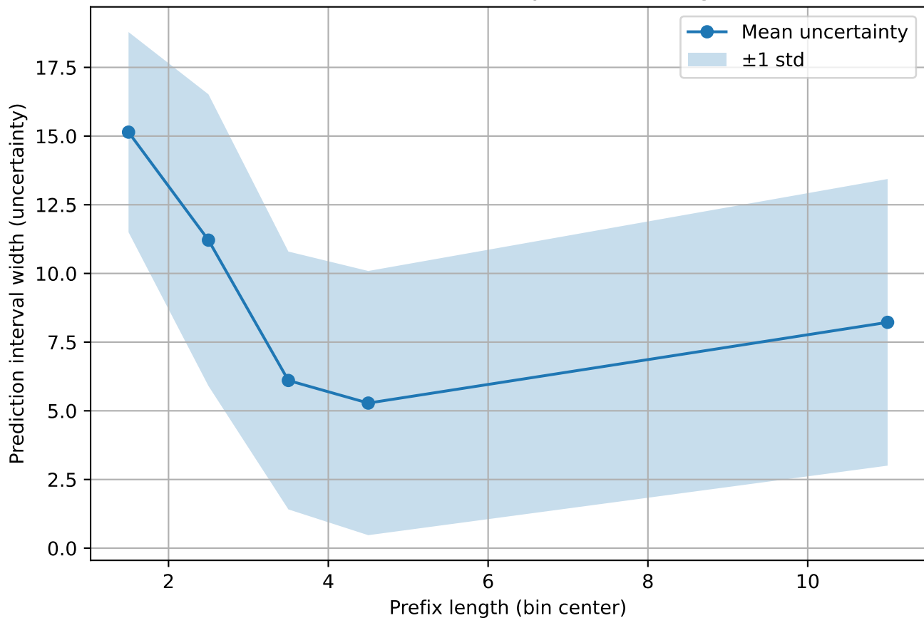
BPIC20DD: Uncertainty vs Prefix Length
